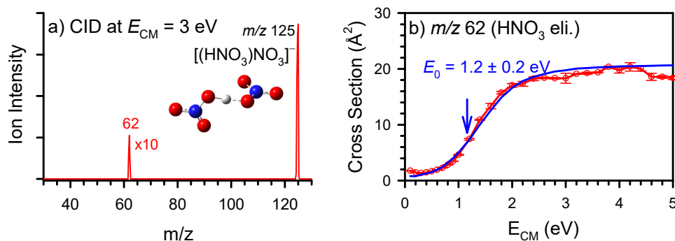
Figure 5 (a) Structure and a representative CID product ion mass spectrum for [(\text{HNO}_3)\text{NO}_3]^- , wherein product ion intensity is scaled by a factor of 10; and (b) product ion cross section as a function of E_{\text{CM}} , wherein the red line with error bars represents the experimental data and the blue line represents the LOC fit.
