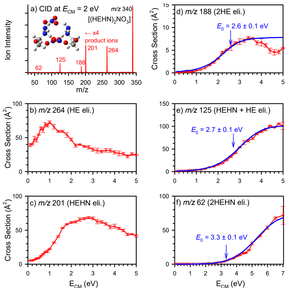
Figure 3 (a) Structure and a representative CID product ion mass spectrum for [(\text{HEHN})_2\text{NO}_3]^- , wherein product ion intensities are scaled by a factor of 4; and (b – f) individual product ion cross sections as a function of E_{\text{CM}} , wherein the red lines with error bars represent the experimental data and the blue lines represent the LOC fits.
